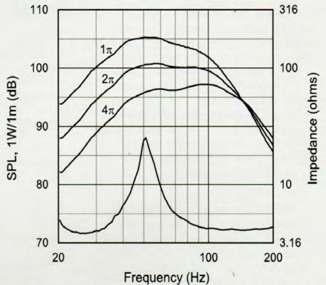
4642A frequency response and impedance (bottom curve), 1 watt at 1 meter, with 150 Hz Linkwitz-Riley 4th order low-pass filter measured under 4\pi ground plane conditions. 1\pi (upper curve) and 2\pi (center curve) loading condition predictions also shown.
