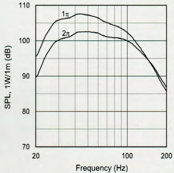
4642A frequency response, 1 watt at 1 meter, with 150 Hz Linkwitz-Riley 4th order low-pass filter and 2nd order high-pass filter at 25 Hz with Q=2 . 1\pi (upper curve) and 2\pi (lower curve) conditions.
